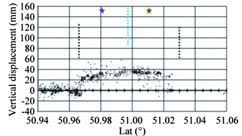
Fig. 4. Variation of the total surface movement along a north-south transect, situated around a longitude of 5.495°E for a 3-year period from August 1992 through August 1995.
